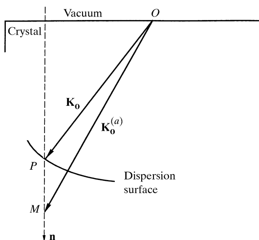
Fig. 5.1.2.2. Boundary condition for wavevectors at the entrance surface of the crystal.
