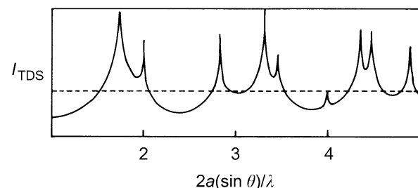
Fig. 7.4.2.4. One-phonon scattering calculated for polycrystalline nickel of lattice constant a (after Suortti, 1980).
