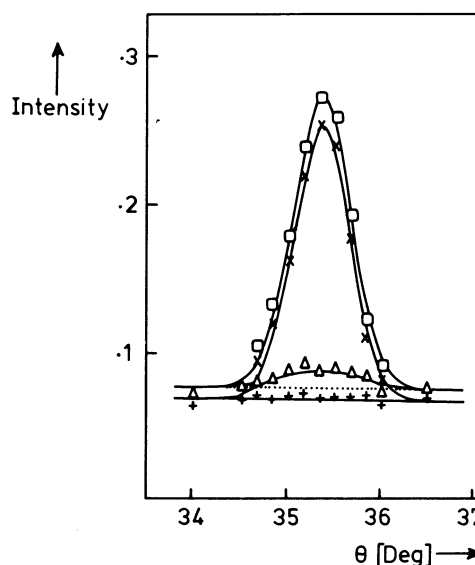
Fig. 7.4.2.1. 060 reflection of \text{LiNbO}_3 (Mössbauer diffraction). Inelastic (triangles), elastic (crosses), total (squares) and background (pluses) intensity (after Krec, Steiner, Pongratz & Skalicky, 1984).
