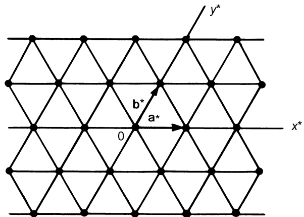
Fig. 9.2.1.9. The a^*b^* reciprocal-lattice net for close-packed layer stackings.
