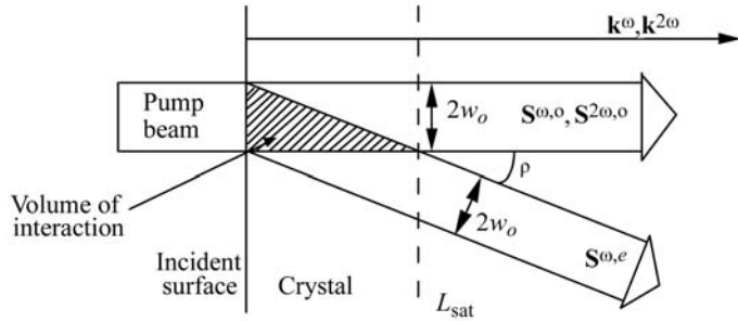
Fig. 1.7.3.9. Beam separation in the particular case of type-II ( oeo ) SHG out of the xy plane of a positive uniaxial crystal or in the xz and yz planes of a positive biaxial crystal. S^{\omega,o} , S^{\omega,e} and S^{2\omega,o} are the fundamental and harmonic Poynting vectors; k^{\omega} and k^{2\omega} are the associated wavevectors collinear to the CPM direction. w_o is the fundamental beam radius and \rho is the walk-off angle. L_{sat} is the saturation length.
