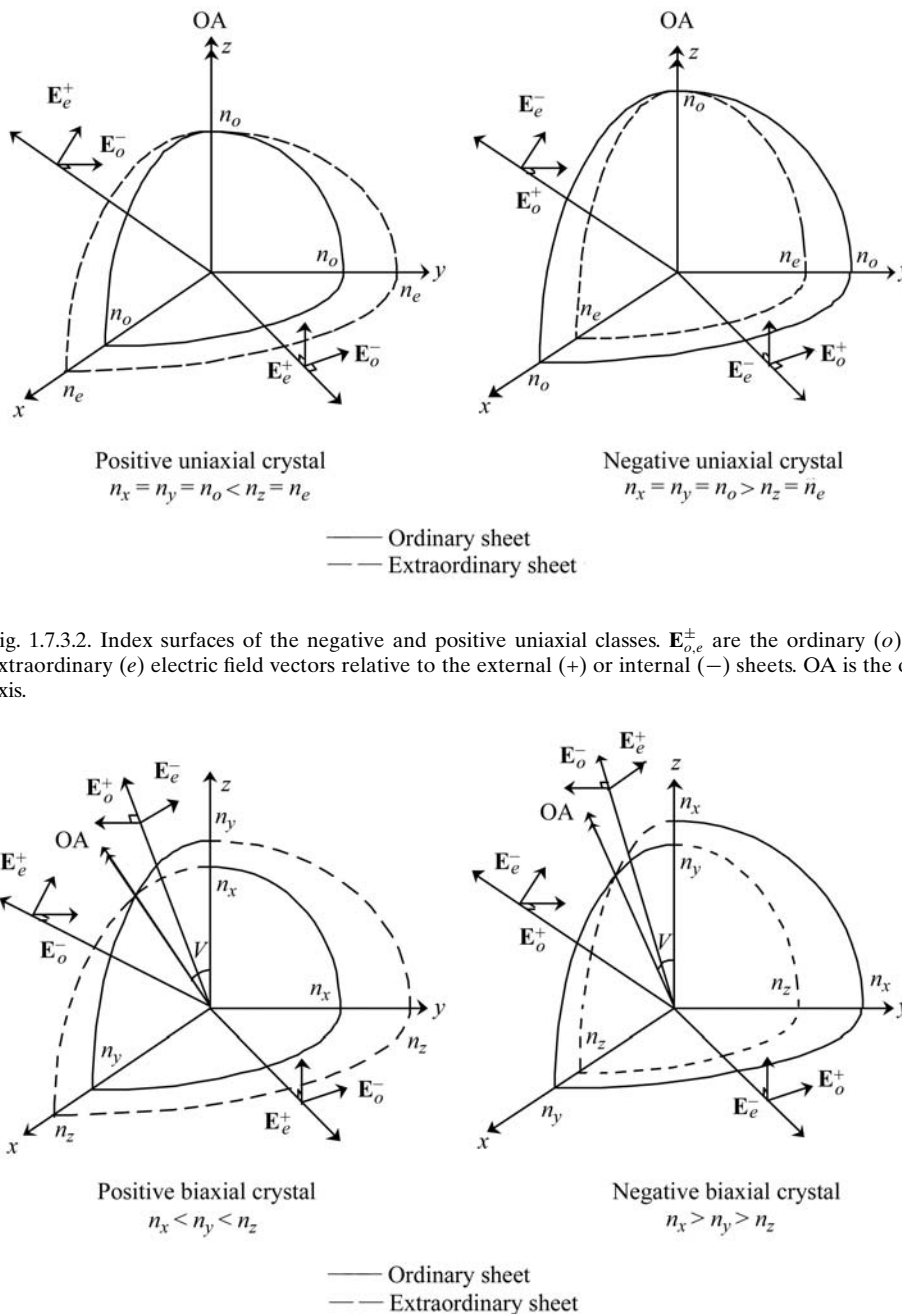
Fig. 1.7.3.3. Index surfaces of the negative and positive biaxial classes. \mathbf{E}_{o,e}^\pm are the ordinary ( o ) and extraordinary ( e ) electric field vectors relative to the external (+) or internal (–) sheets for a propagation in the principal planes. OA is the optic axis.
