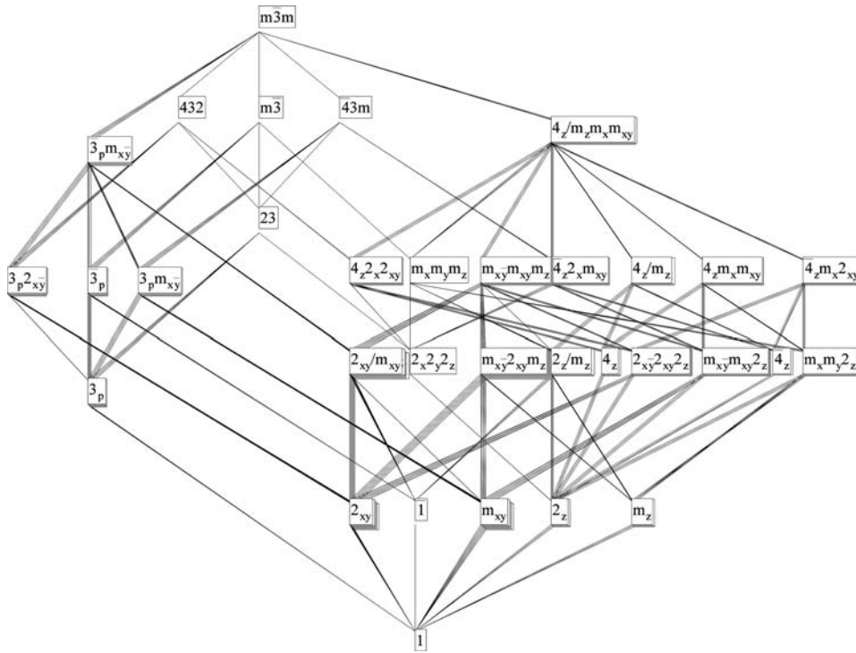
Fig. 3.1.3.1. Lattice of subgroups of the group \bar{m}3m . Conjugate subgroups are depicted as a pile of cards. In the software GI*KoBo-1 , one can pull out individual conjugate subgroups by clicking on the pile.
