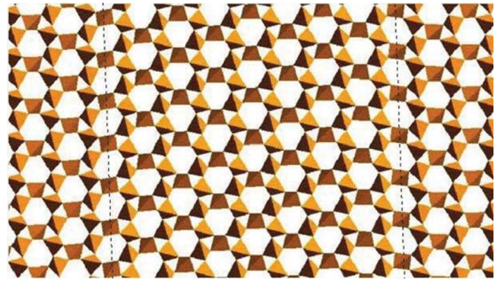
Fig. 3.4.4.4. Microscopic structure of two domain states and two parallel mutually reversed domain walls in the \alpha phase of quartz. The left-hand vertical dotted line represents the domain wall \mathbf{W}_{12} , the right-hand line is the reversed domain wall \mathbf{W}_{21} . To the left of the left-hand line and to the right of the right-hand line are domains with domain state \mathbf{S}_1 , the domain between the lines has domain state \mathbf{S}_2 . For more details see text. Courtesy of M. Calleja, University of Cambridge.
