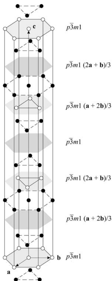
Fig. 5.2.5.2. The structure of cadmium chloride, CdI 2 . The section planes of two orbits in special positions are distinguished by shading. Notice the different location of the sectional layer groups on different levels for the same orbit. The figure is drastically elongated in the c direction to exhibit the layer symmetries.
