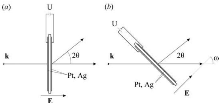
Figure 2.8.4 In situ transmission geometry developed by Schönau, Schmitt et al. (2007) with the electric field vector perpendicular to the flat-plate sample surface. The electric field results from an applied voltage U between two opposing sputtered electrodes (Ag, Pt) with a thickness of about 15 nm. (a) \omega = 0^\circ and (b) \omega = 45^\circ .
