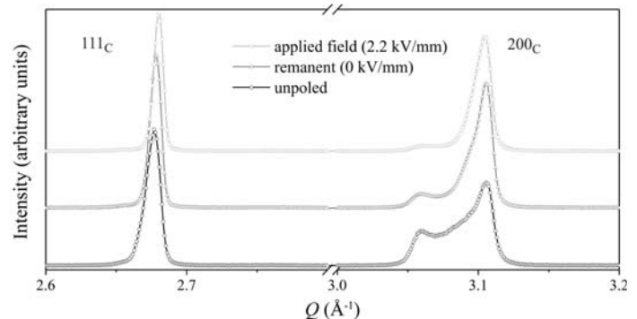
Figure 2.8.5 111_C and 200_C reflections of the unpoled, remanent and applied field state of PIC 151 at \omega = 0^\circ . Owing to the piezoelectric effect, the 111_C reflection is shifted. The preferred orientation of the 200_C reflection indicates tetragonal 90^\circ domain switching.
