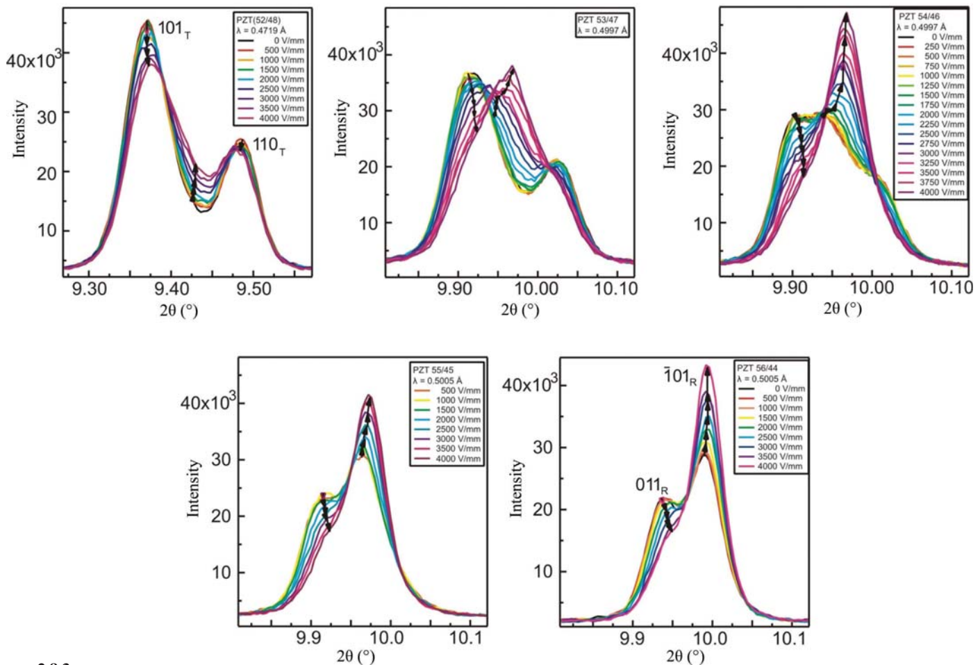
Figure 2.8.3 Diffraction patterns of the tetragonal 101_T/110_T reflection pairs of PZT 52/48, PZT 53/47, PZT 54/46, PZT 55/45 and PZT 56/44 recorded in situ under an electric field for the first poling cycle of up to 4 \text{ kV mm}^{-1} . Reproduced with permission from Schönau, Knapp et al. (2007). Copyright (2007) by the American Physical Society.
